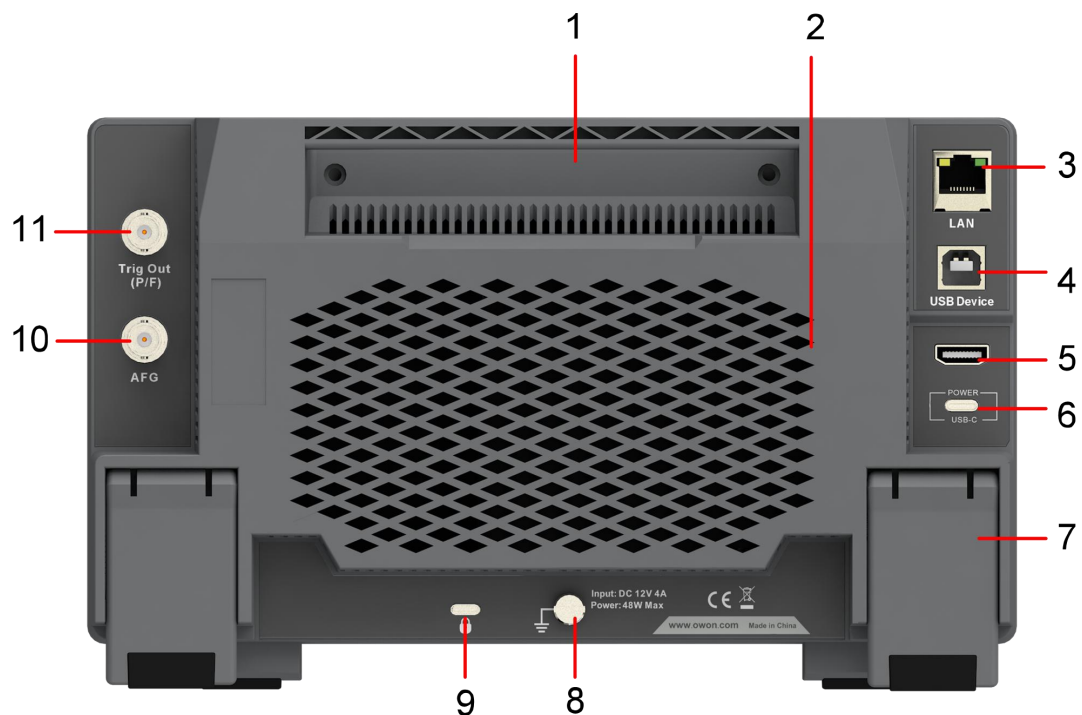
Figure 3-2: Rear Panel
