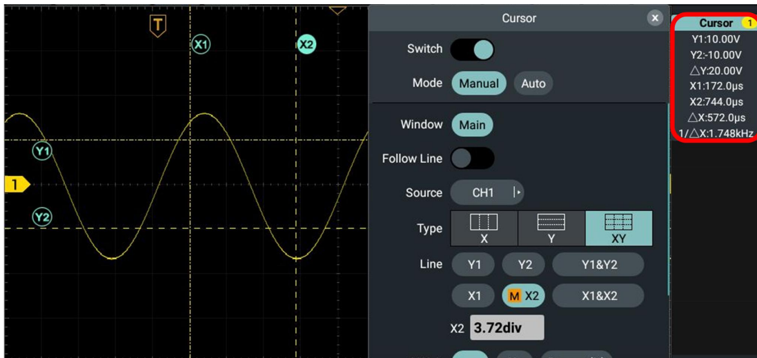
Figure 5-8:Time &Voltage Cursor Measurement
